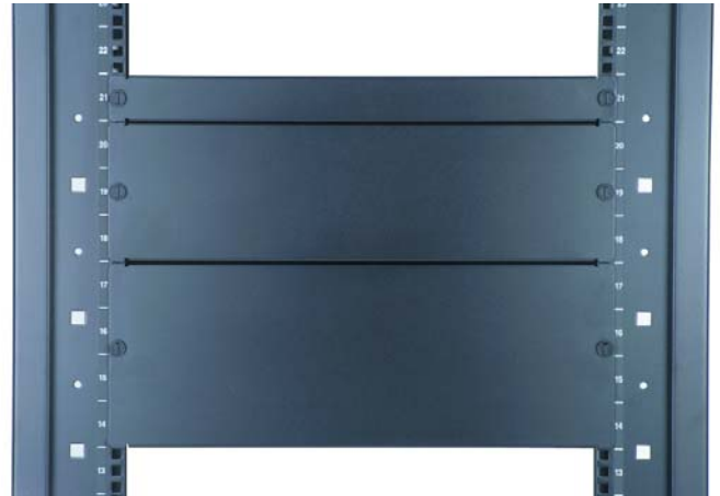
1U, 3U and 4U Tool-less Blanking Panels installed in a rack with 0.375" Mounting Angles
